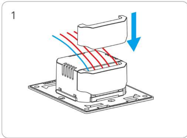
Install the protective cover.
