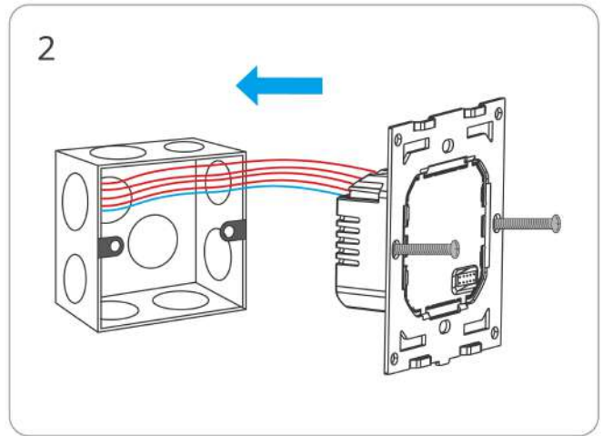
Tighten the power module to the mounting box with screws.
