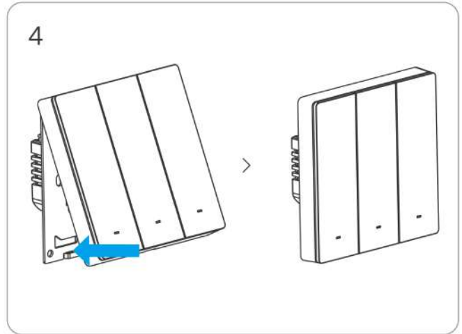
Press downward to fix the switch module in place, it will automatically align with the pin positions.
